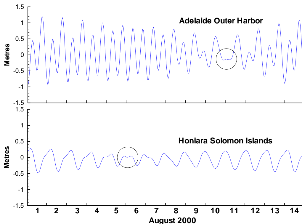
Figure 3 Sea levels at Adelaide and Honiara. Intervals with virtually no tidal variation are encircled. In Adelaide these intervals are called the "Dodge Tide".
