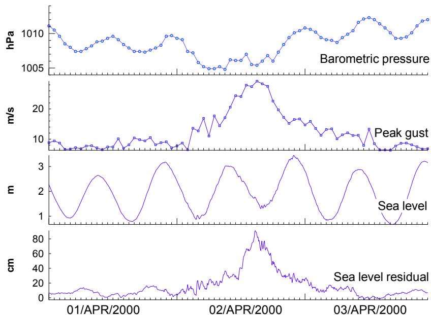
Figure 6 Weather and water level data recorded by the National Tidal Centre (Bureau of Meteorology) SEAFRAME gauge at Cape Ferguson. Barometric pressure and peak gust are recorded on the hour; sea level is recorded at six minute intervals. Time is UT.
