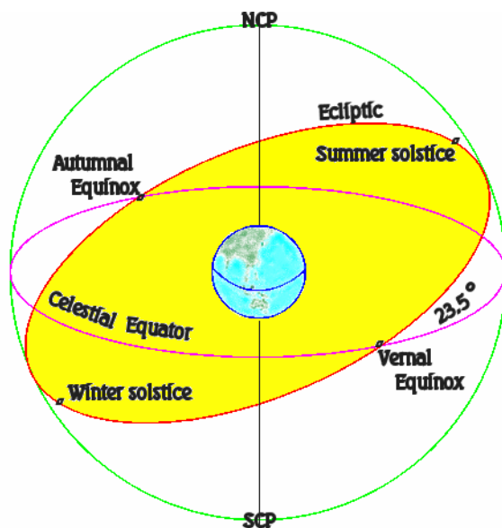
Figure 2 The celestial sphere, as seen from on high, far out in the starry heavens.
