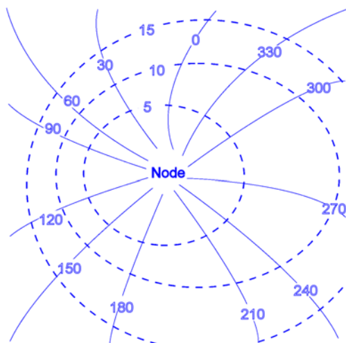
Figure 1 A schematic of an amphidrome. Dashed lines show amplitude (cm), increasing away from the node. Solid lines show phase (degrees), increasing counter-clockwise around the amphidrome (typical of northern hemisphere amphidromes).
