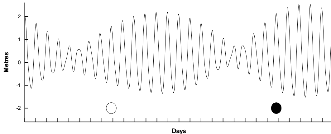
Figure 11 Predicted tidal heights at Karumba, Queensland (latitude 17° 29' S) over a one month period. Full and new moons are indicated. The beat cycle is caused by O_1 and K_1 .
