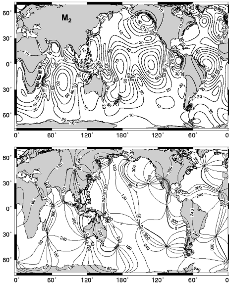
Figure 6 The "SAL tide" for M_2 : ( top ) Amplitude contours in mm; ( bottom ) phase lag (degrees, UT). The phase contours are broadly similar to those seen on maps of the global M_2 tide. Graphic courtesy of Richard Ray. (Note that the SAL function is mathematically defined over land, but is not physically meaningful except over oceans and large lakes.)
