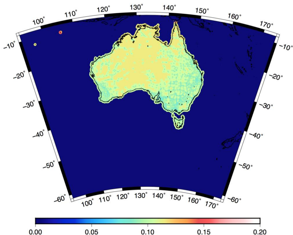
Figure 9: (top) One standard deviation of AGQG uncertainty. Units in metres. (bottom) One standard deviation of AUSGeoid2020 uncertainty. Units in metres from Brown et al. (2018).
